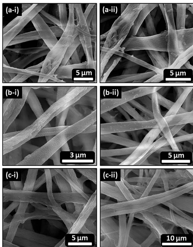
Fig. 8 Representative SEM micrographs of the (a-i and a-ii) A. eucrenophila , (b-i and b-ii) C. michiganensis and (c-i and c-ii) P. aeruginosa immobilized CA web after the reusability tests, showing attachment of bacterial biofilms on fiber surfaces.
