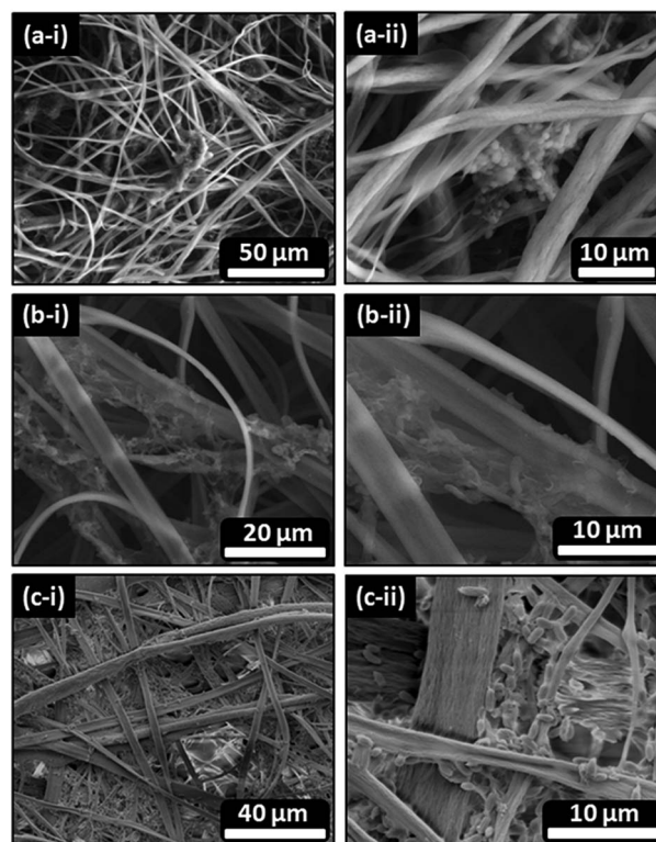
Fig. 4 Representative SEM images of CA nanofibrous web after immobilization of (a-i and a-ii) Aeromonas eucrenophila , (b-i and b-ii) Clavibacter michiganensis , (c-i and c-ii) Pseudomonas aeruginosa after 7 days.
