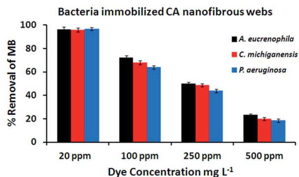
Fig. 6 The effect of initial dye concentration on the decolorization yield of the bacteria immobilized CA nanofibrous web during the 48 h incubation period (pH 7; T: 30 °C; stirring rate: 100 rpm). Error bars represent the means of three independent replicates.
