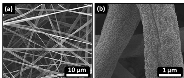
Fig. 2 Representative SEM images of electrospun CA nanofibrous web (a) low magnification, and (b) high magnification.
