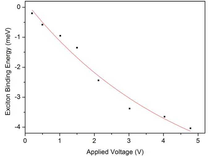
FIG. 6. Exciton binding energy as a function of applied voltage. Dots represent the obtained binding energies from calculations at given bias voltages.
