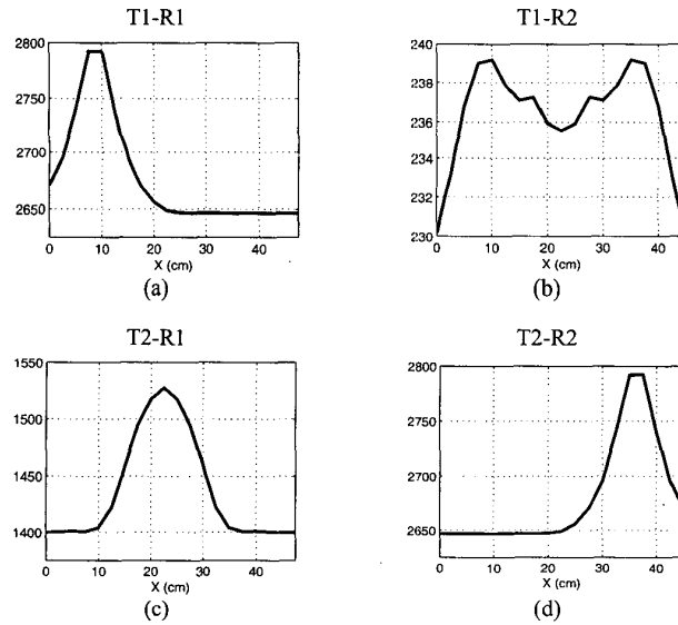
Figure 2: Received-signal energy vs. the position of the target. The target is a conducting prism buried 8 cm under the ground.
