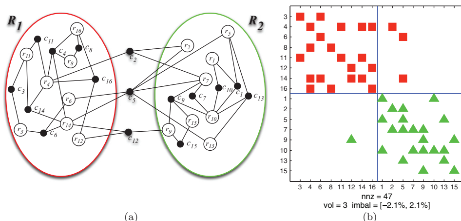
FIG. 3.3. First step of 4-way jagged-like partitioning of the matrix shown in Figure 2.1: (a) 2-way partitioning \Pi_R of column-net hypergraph representation \mathcal{H}_R of \mathbf{A} ; (b) 2-way rowwise partitioning of matrix \mathbf{A}^{\Pi} obtained by permuting \mathbf{A} according to the partitioning induced by \Pi ; the nonzeros in the same partition are shown with the same shape and color; the deviation of the minimum and maximum numbers of nonzeros of a part from the average are displayed as an interval \text{imbal} ; \text{vol} denotes the number of nonzeros and the total communication volume.
