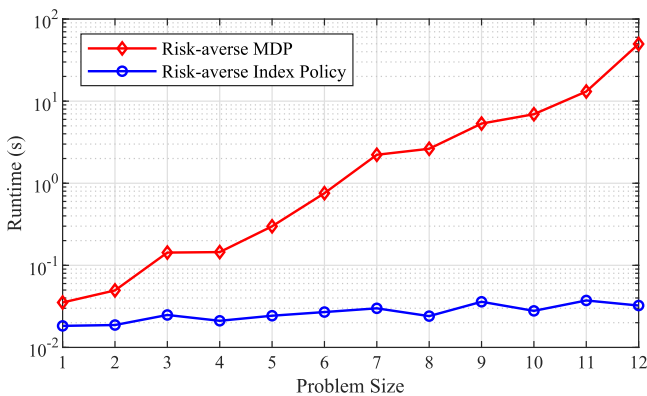
Fig. 1. Runtime of obtaining the optimal policy and index policy for first-order mean-semideviation.
