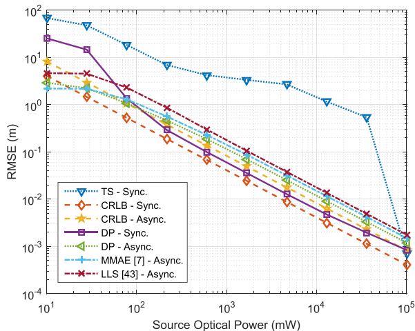
Fig. 12. CRLBs and RMSEs of the estimators for two-dimensional localization in synchronous and asynchronous VLP systems with respect to source optical power, where T_s = 1 \mu s and f_c = 100 MHz.
