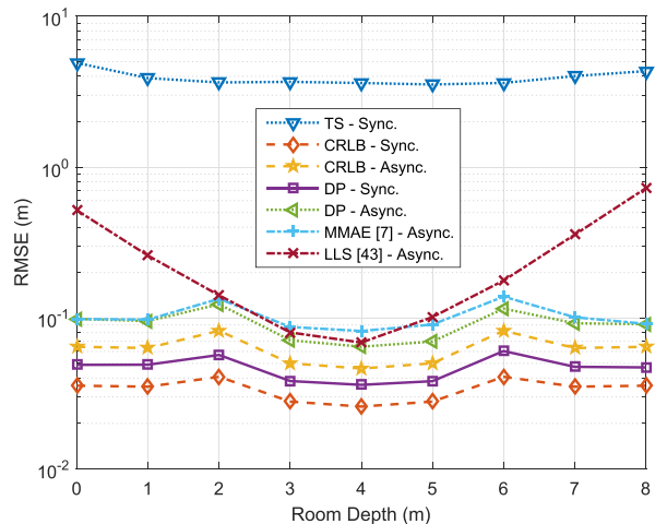
Fig. 13. CRLBs and RMSEs of the estimators for two-dimensional localization in synchronous and asynchronous VLP systems with respect to room depth, where T_s = 1 \mu s , A = 1 W and f_c = 100 MHz.
