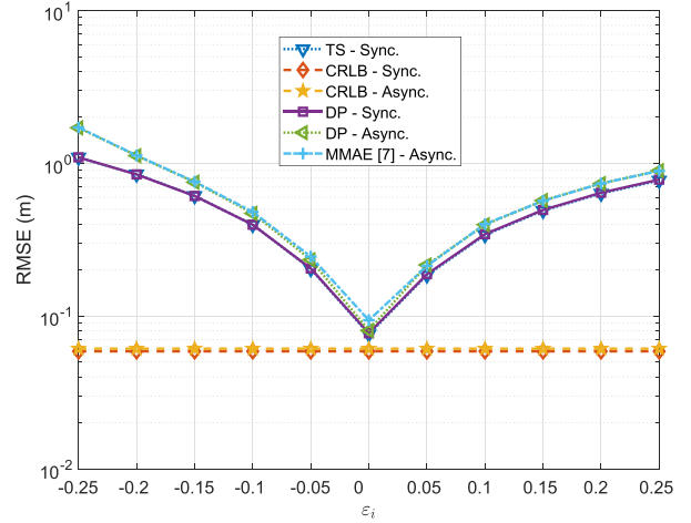
Fig. 11. CRLBs and RMSEs of the estimators for synchronous and asynchronous VLP systems under mismatched transmission model, where T_s = 1 \mu\text{s} , A = 1 \text{ W} , and f_c = 10 \text{ MHz} .
