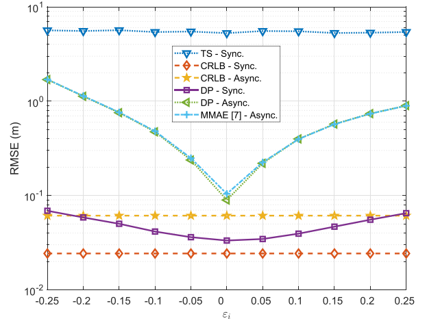
Fig. 10. CRLBs and RMSEs of the estimators for synchronous and asynchronous VLP systems under mismatched transmission model, where T_s = 1 \mu\text{s} , A = 1 \text{ W} , and f_c = 100 \text{ MHz} .
