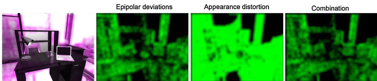
Fig. 17 Optical flow performance. We adapted the optical flow method proposed in [1] to detect and localize specular objects. Shown is a sample frame from the computer-rendered test set with an overlaid epipolar deviation field, that exhibits very poor specificity. In addition, appear-
