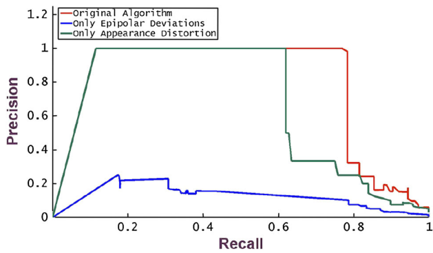
Fig. 13 Individual contributions of cues. A Precision-Recall curve for the algorithm (red) and individual cues (blue epipolar deviation, green appearance distortion). The specular object was of medium size, the camera trajectory, rotation in azimuth
