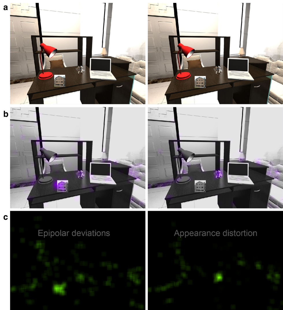
Fig. 4 Epipolar deviation vs. appearance distortion: specificity. Moving, diffusely reflecting objects, such as the photograph of the house in the above scene, will distort the optic flow field solely due to camera motion. This will cause epipolar deviations, which a specular detection algorithm, that is solely based on this cue, may label as specular. a An office scene. In addition to camera motion the photograph, located on the desk, moves. b Left this causes large epipolar deviations ( purple overlay), thus this region would incorrectly be labeled as specular. Right appearance distortion ( purple overlay) is not affected by this manipulation and correctly labels the specular object. c Epipolar deviation and appearance distortion for this sequence
