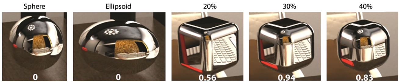
Fig. 11 Effect of 3D shape. Specular object shapes tested: sphere , ellipsoid and chamfer box with three different edge curvatures. Precision of the detection algorithm are shown as inset in each subpanel
