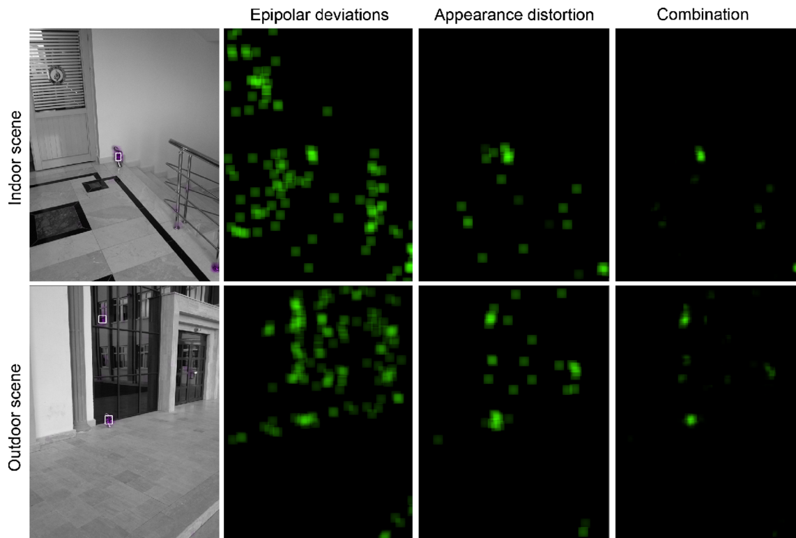
Fig. 15 Real video sequences. Two frames of indoor (hallway) and outdoor (building) videos are shown in the left most column, along with corresponding epipolar deviation-, appearance distortion-, and combined specularity fields (from left to right). The white bounding box overlaid on the original frame (left column) show that the specular object was successfully localized using the combined cue. Color codes are as in
