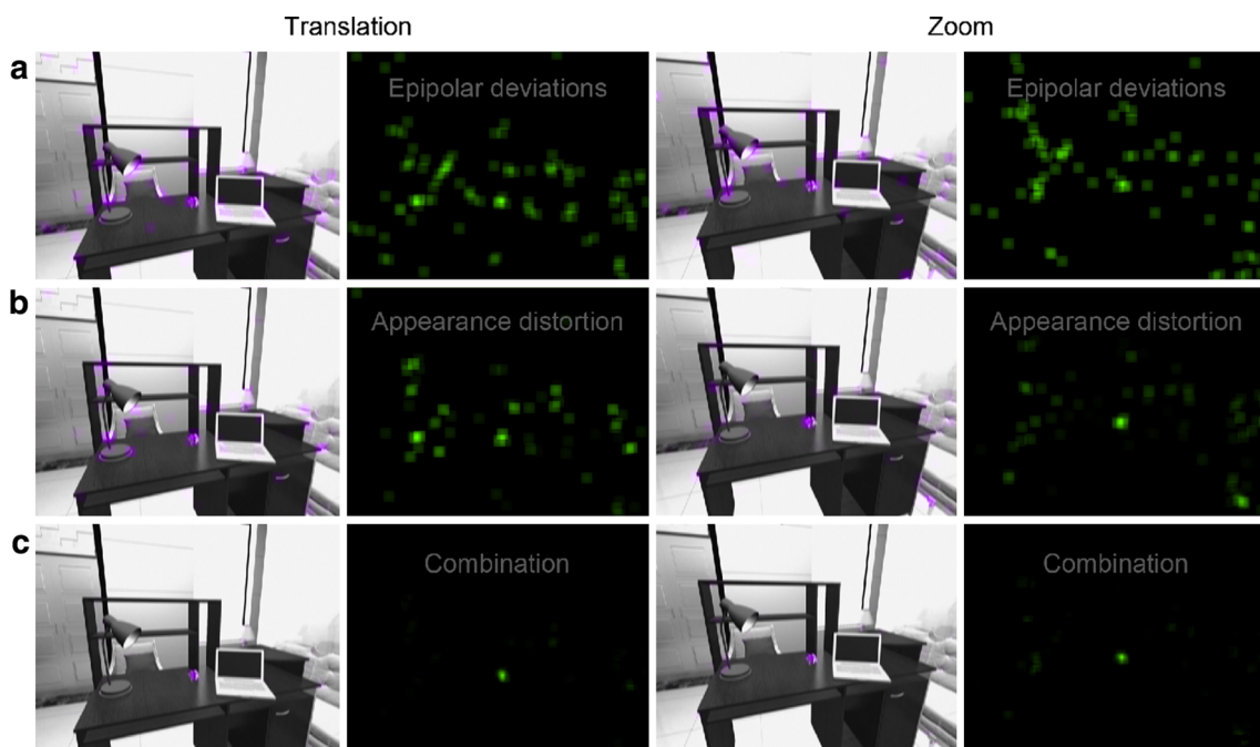
Fig. 14 Performance boost through combination of cues. The combination of epipolar deviation row (a) and appearance distortion (b) significantly enhances specularity detection performance of the algorithm
