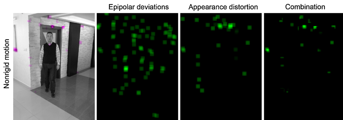
Fig. 16 Real video sequences—nonrigid motion. We tested whether the video of a walking person causes false alarms in specularity detection, due to the potentially substantial amount of appearance distortion and epipolar deviations. Yet, the algorithm proved robust under this condition and did not label any regions as specular in these video sequences,
