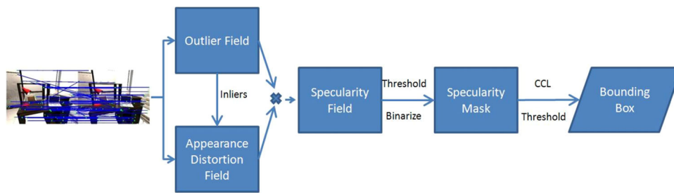
Fig. 6 Flowchart of the algorithm. After applying SIFT, matching outlier and appearance distortion fields are obtained. These two fields are multiplied pixel by pixel to yield the specularity field. A specularity mask is created by thresholding the specularity field. Connected com-
