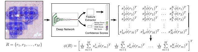
Fig. 6. ROI-level deep feature representation computed by pooling the final patch-level deep feature representations.
