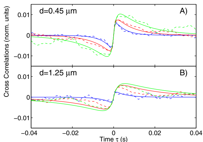
Fig. 4: (Color online) Cross-correlation function for an optically trapped particle whose diameter is (a) 0.45 \mu\text{m} and (b) 1.25 \mu\text{m} . The powers used are listed in table 1 and the color legend is P (blue) > P (red) >> P (green). Dashed lines represent experimental data, while solid lines are the curves obtained from the fit.
