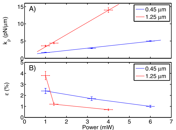
Fig. 5: (Color online) (a) Behavior of the radial stiffness k_\rho as a function of the laser power for the two kinds of particle used. The solid lines are the linear fits. (b) Value of the relative contribution of the non-conservative component \epsilon as a function of the power used. Notice that it increases for lower powers.
