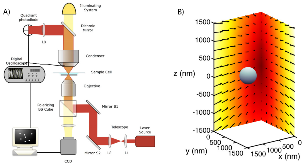
Fig. 1: (Color online) (a) Schematics of the experimental setup. (b) Forces acting on a colloidal particle held by an optical trap. The lines represent the force-field and the color represents the modulus of the force. A slight bending of the force lines due to the non-conservative component of the force-field can be observed (see also fig. 2).
