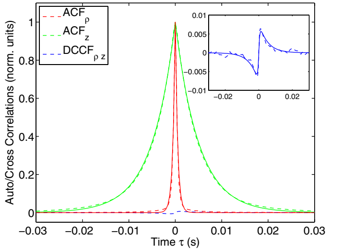
Fig. 3: (Color online) Autocorrelation functions (ACFs) and difference of the cross-correlation function (DCCF) for a 0.45 \mu\text{m} colloidal particle optically trapped with a laser power of 6 mW at sample (first line of table 1). Inset: Closeup of the DCCF. Dashed lines represent experimental data, while solid lines are the curves obtained from the fit with eqs. (4)–(6).
