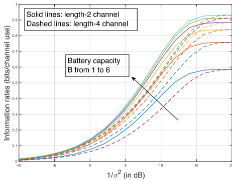
Fig. 4. Information rates of 2-tap and 4-tap channels in the previous example for different battery capacities.
