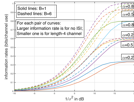
Fig. 5. Information rates for three different energy arrival rates.
