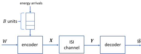
Fig. 1. EH communication over an ISI channel.
