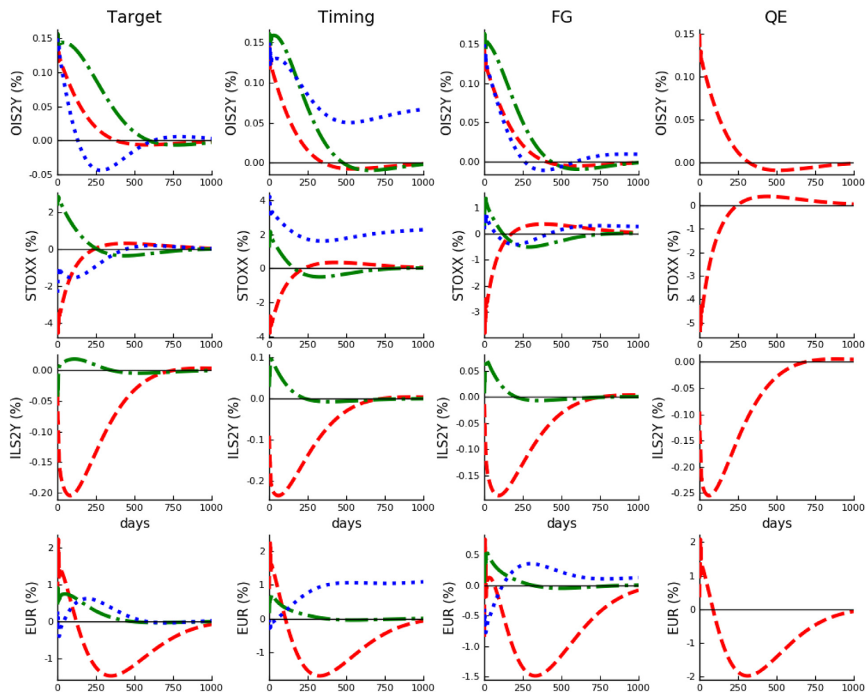
Fig. 5. Financial VAR.
