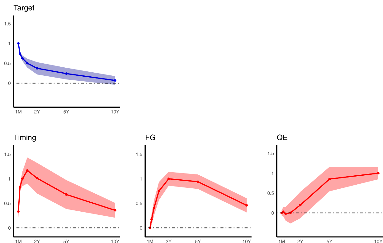
Fig. 3. Factor loadings.
