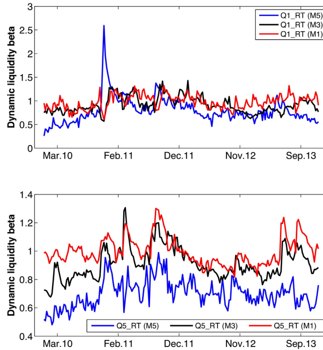
Fig. 2. Selected time varying liquidity betas for different firm size quintiles ( M5 : largest firms, M1 : smallest firms) estimated by Dynamic Conditional Beta methodology: (a) for smallest position ( Q1 ) to roundtrip; (b) for largest position ( Q5 ) to roundtrip.
