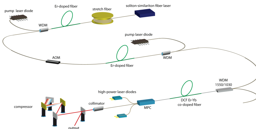
Fig. 1. Schematic drawing of the experimental setup; MPC, multiple pump signal combiner; DCF, double-clad fiber, WDM, wavelength-division multiplexer.
