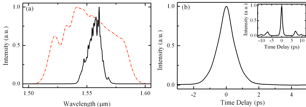
Fig. 2. (a) Measured optical spectra of the seed (red, dashed line) and the 2 \mu\text{J} , amplified output (black, solid line). (b) Measured autocorrelation result after dechirping yielding 700-fs pulse duration with 0.5 \mu\text{J} energy. Inset shows long-range autocorrelation where the satellite pulses are due to birefringence of the AOM.
