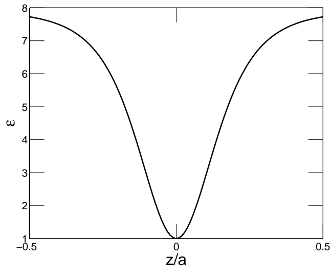
Figure 4. Same with Fig.3 but for the position dependence of the dielectric function of the one dimensional vortex lattice within a spatial period.
