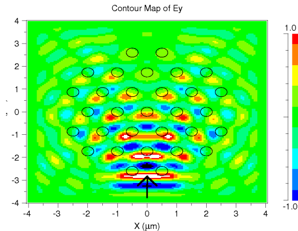
Figure 9. Same finite vortex lattice as in Fig.8, but rotated by \pi/6 . A directional band gap is clearly seen as there is no transmission.
