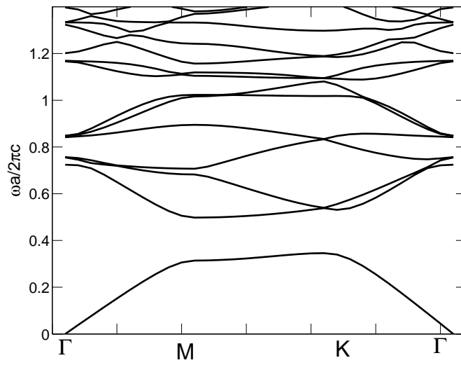
Figure 6. TE band structure of a triangular vortex lattice with a = 4.5\xi of N = 5.5 \times 10^{20}\text{m}^{-3} ^{87}\text{Rb} atoms ( a_{sc} = 5.5\text{nm} , \lambda = 794\text{nm} ).
