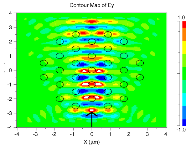
Figure 8. A vortex lattice with 31 vortices. Vortex spacing is taken to be 5 times the vortex core size which is equal to the light wavelength. Vortex cores have n = 1 while BEC has index of refraction n = 3 . With these parameters infinite lattice results indicate a directional band gap, which can be observed by comparing this figure with the Fig.9. Direction of the incident light is denoted by an arrow in both figures.
