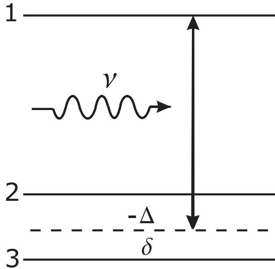
Figure 1. Three-level atom interacting with a field of frequency \nu . The optical field detuned from the resonant transitions by \Delta = \omega_{12} - \nu and \delta = \omega_{13} - \nu .
