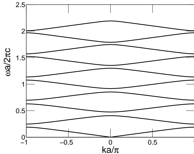
Figure 3. Band structure of a one dimensional vortex lattice of ^{87}\text{Rb} with N = 5.5 \times 10^{20} \text{m}^{-3} and a = 10\xi .
