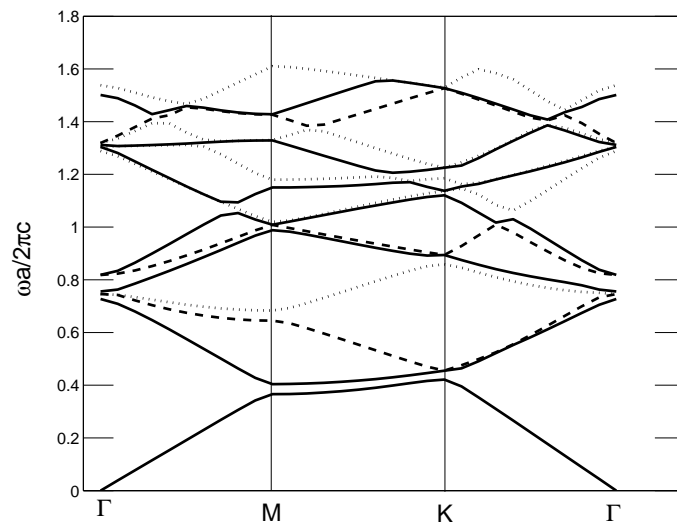
Figure 5. TE band structure of a triangular vortex lattice with a = 10\xi of N = 6.6 \times 10^{20} \text{m}^{-3} ^{23}\text{Na} atoms. Different line patterns are used for visual clarity.
