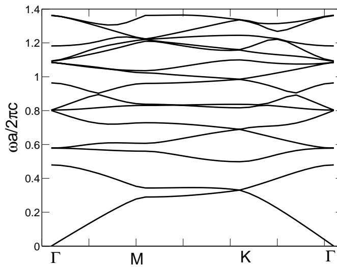
Figure 7. Same with Fig.6 but for the TM band structure
