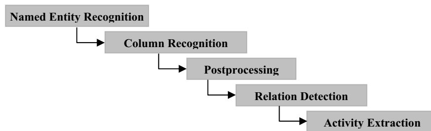
Fig. 3. General flow of the tasks performed by the Extractor.
