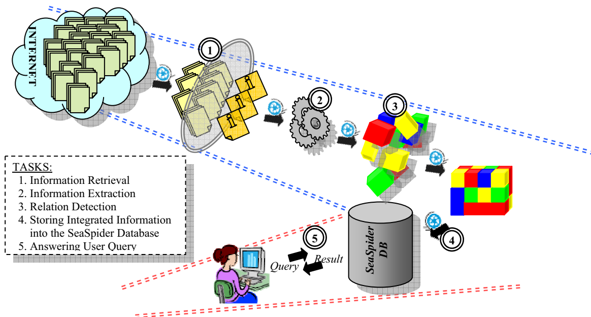
Fig. 1. The general flow of the SeaSpider.
