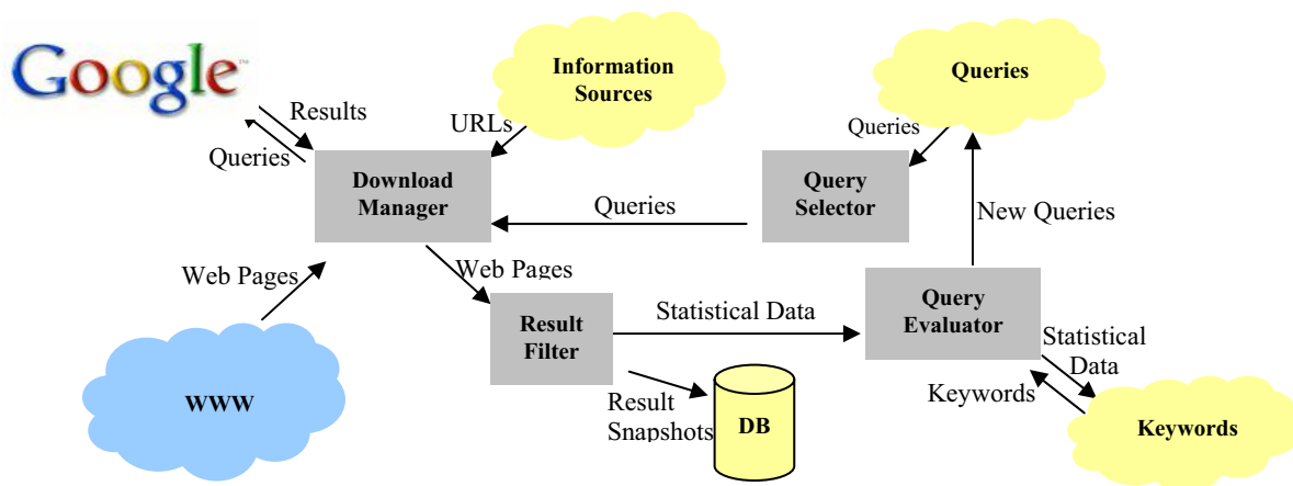
Fig. 2. The Retrieval Engine.
