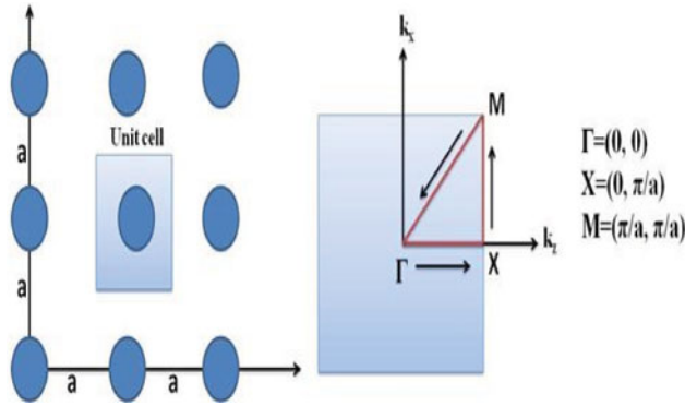
Figure 1. Unit cell and associated Brillouin zone for square lattice (Color figure available online).
