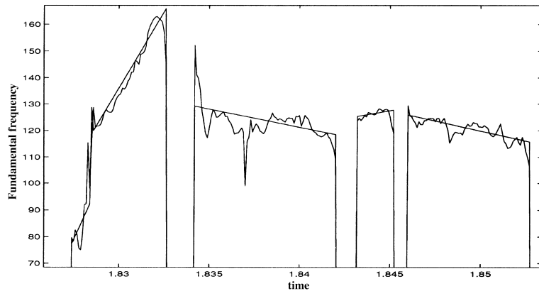
Fig. 3. F0 contour filtering and regularization.
