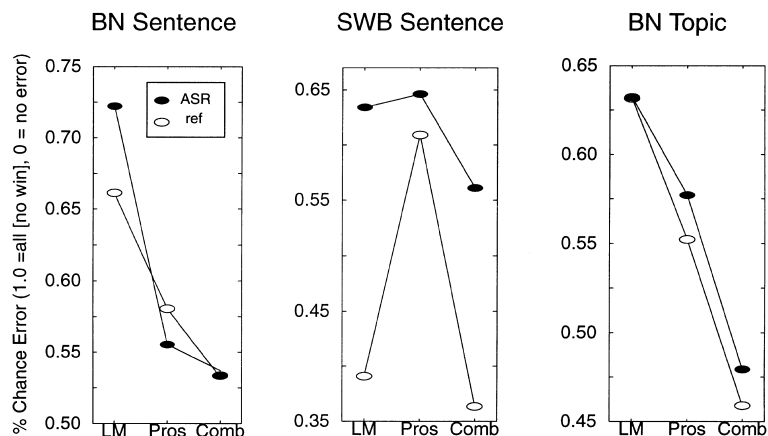
Fig. 9. Percentage of chance error remaining after application of model (allows performance to be directly compared across tasks). BN = Broadcast News, SWB = Switchboard, ASR = 1-best recognition hypothesis, ref = transcribed words, LM = language model only, Pros = prosody model only, Comb = combination of language and prosody models.
