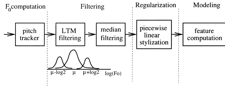
Fig. 2. F0 processing.
