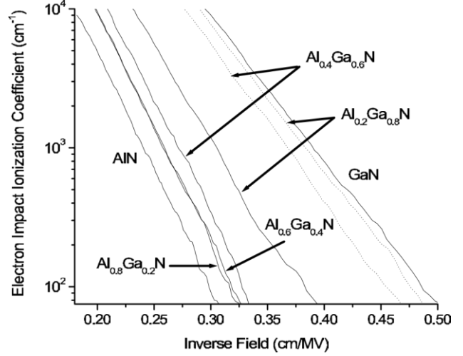
Figure 1. Electron II coefficient versus inverse electric field. Dotted curves indicate the results when alloy scattering is not included. The curves for \text{Al}_{0.6}\text{Ga}_{0.4}\text{N} and \text{Al}_{0.8}\text{Ga}_{0.2}\text{N} merge at higher fields. These results are obtained for a temperature of 300 K and an ionized impurity concentration of 10^{17} \text{ cm}^{-3} .
