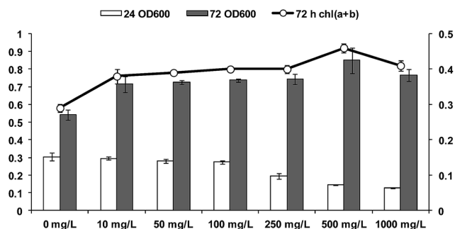
Fig. 2 Interactive effect on optical density ( \text{OD}_{600} ) and chlorophyll content of Chlorella sp. with \text{La}_2\text{O}_3 NP during the incubation period (24 and 72 h). The diagram represents algal growth inhibition at 24 h exposure and growth enhancement observed at 72 h. Results are mean values of triplicate cultures.
