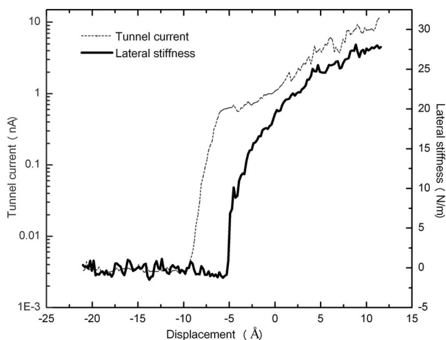
FIG. 5. Simultaneous lateral-force gradient-distance and tunnel current vs distance spectroscopy. The sample bias voltage was set on -1 V. The cantilever free-oscillation amplitude is 0.4 \text{ \AA}_p . This curve was obtained from different sites on the sample away from the position that Fig. 4 was acquired.
