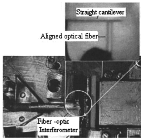
FIG. 1. Photo of the aligned optical fiber at the side of the special cantilever to measure the lever deflections.
