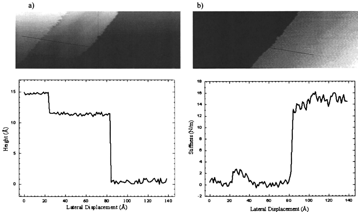
FIG. 3. Simultaneous imaging of Si(111). (a) Topography image and lower curve shows the cross-section view of the STM topography image. (b) Lateral-force gradient image and lower curve shows the cross-section view of the force-gradient image. Image size: 213 \times 80 \text{ \AA}^2 . The lever was oscillated parallel to the surface with an oscillation frequency of 7.56 kHz and oscillation amplitude of 0.4 \text{ \AA}_p . Tip bias voltage and set tunnel current were -1 \text{ V} and 0.4 \text{ nA} , respectively.
