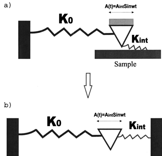
FIG. 2. (a) Schematic view of lateral tip-sample interaction and (b) mass-spring modeling of the tip-sample interaction.
