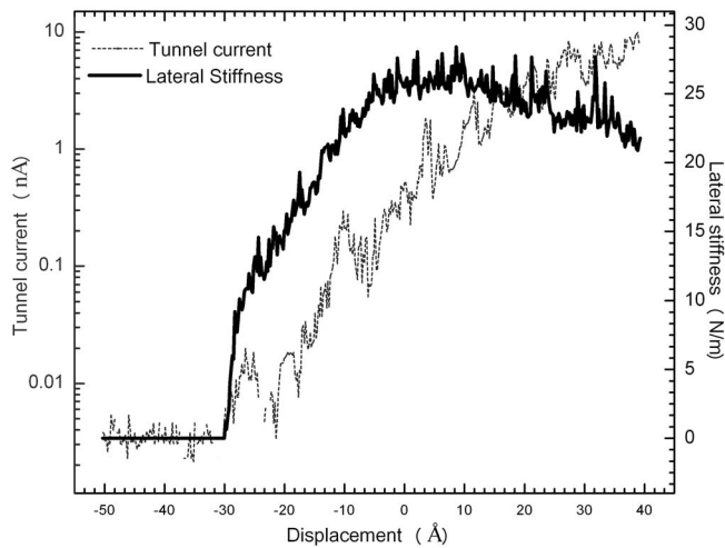
FIG. 4. Simultaneous lateral-force gradient-distance and tunnel current vs distance spectroscopy. The sample bias voltage was set on -1 V. The cantilever free-oscillation amplitude is 0.4 \text{ \AA}_p .
