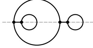
FIGURE 1. The skeleton of \bar{B}
