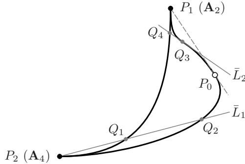
FIGURE 2. The quartic C with the set of singularities \mathbf{A}_4 \oplus \mathbf{A}_2
