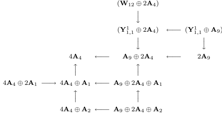
FIGURE 7. Immediate adjacencies of sets of singularities
