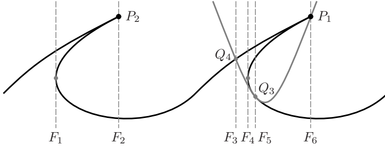
FIGURE 6. The set of singularities \mathbf{A}_9 \oplus 2\mathbf{A}_4 \oplus \mathbf{A}_2
