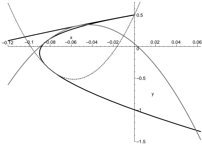
FIGURE 8. Maple plot of the curve \bar{B} (black), a double tangent (solid grey), and an inflection tangent through a singular point (dotted grey)
