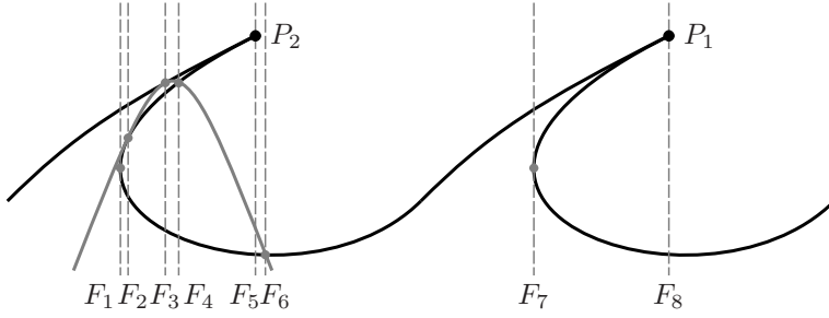
FIGURE 5. The set of singularities 4\mathbf{A}_4 \oplus 2\mathbf{A}_1
