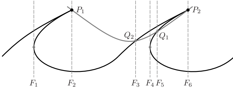
FIGURE 4. The set of singularities 2\mathbf{A}_9
