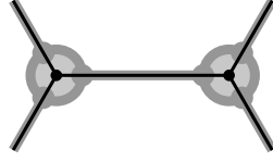
FIGURE 1. A 3-skeleton \text{Sk} (black), auxiliary graph \text{Sk}^\circ (bold grey), and space \text{Sk}^\bullet deformation equivalent to \text{Sk} (bold and light grey)
