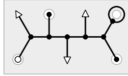
FIGURE 9. A generalized pseudo-tree \text{Sk}^c and punctured disk B^\sharp
