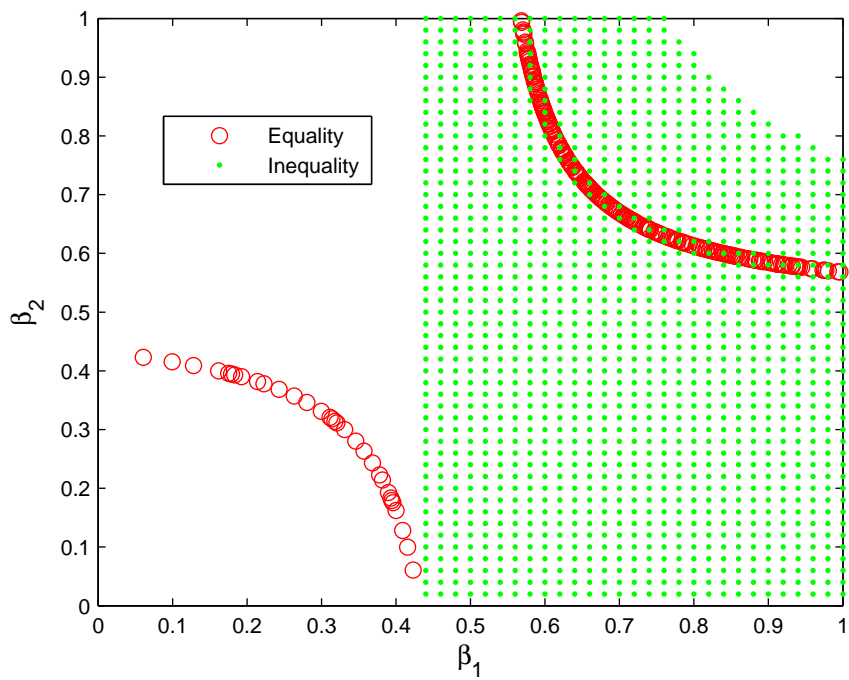
Figure B.2: Feasible regions of (B.5) and (B.6) for \lambda = 2
