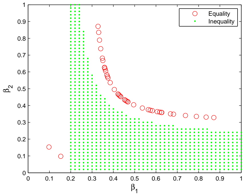
Figure B.4: Feasible regions of (B.5) and (B.6) for \lambda = 5
