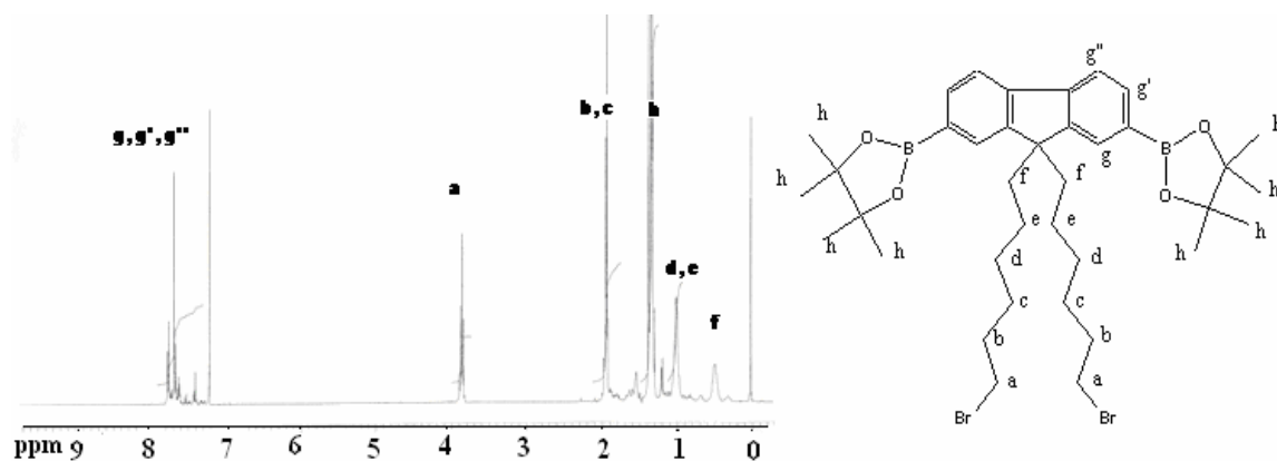
Fig. 2.10- ^1\text{H} -NMR Spectrum of 5 (400 MHz, \text{CDCl}_3 , 25 °C)
