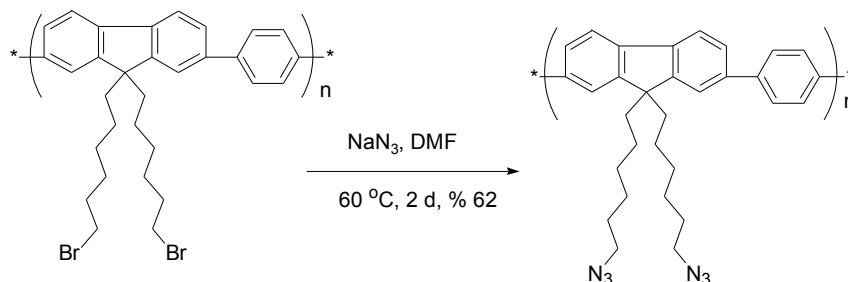
Scheme 2.12- The synthesis of P4
