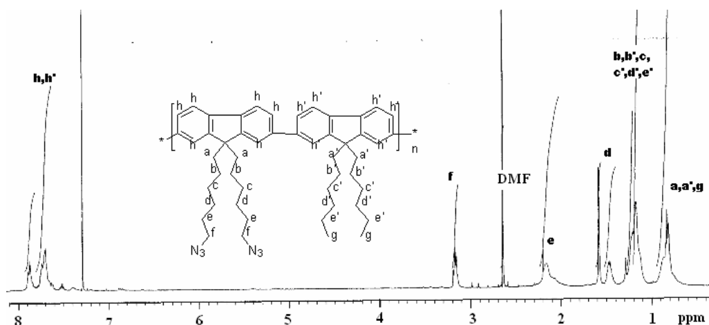
Fig. 2.16- 1 H-NMR spectrum of P2 (400 MHz, CDCl 3 , 25 °C)
