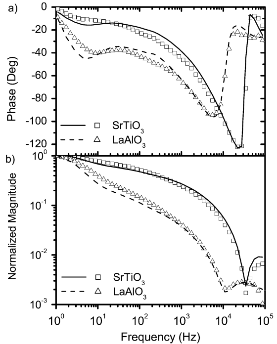
Fig. 4. (a) Phases and (b) magnitudes of pixels C on LaAlO 3 and SrTiO 3 substrates and their fitting curves.
