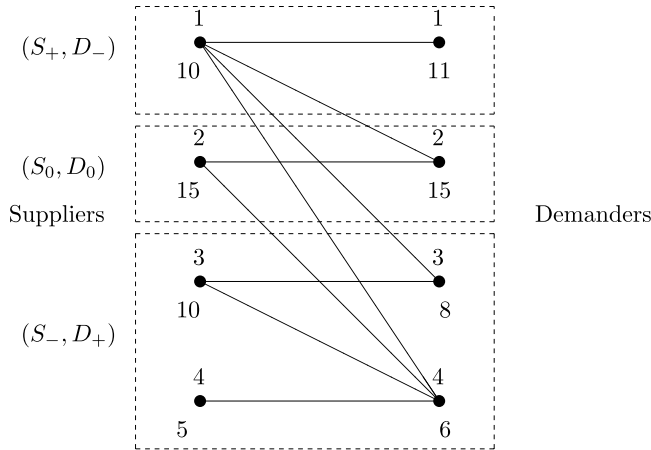
FIGURE 4. Decomposition with a balanced subgraph.
