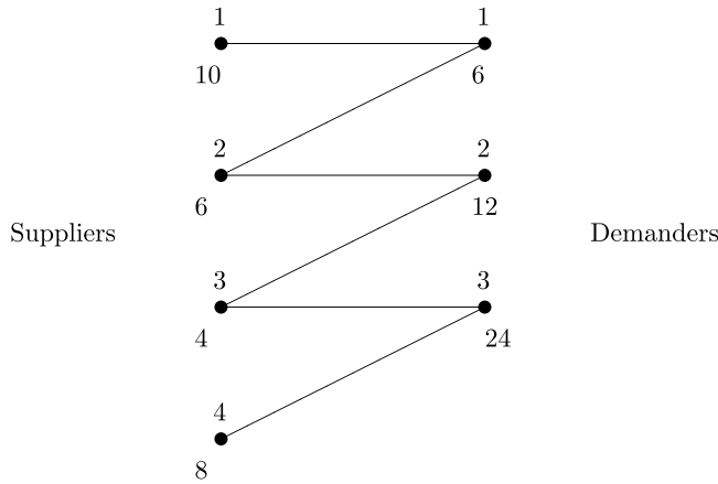
FIGURE 1. Short supply and short demand co-exist.
