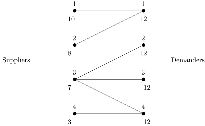
FIGURE 2. Agents on the short side are not treated identically.
