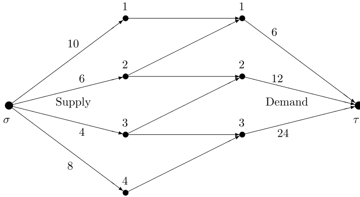
FIGURE 3. The max-flow problem.
