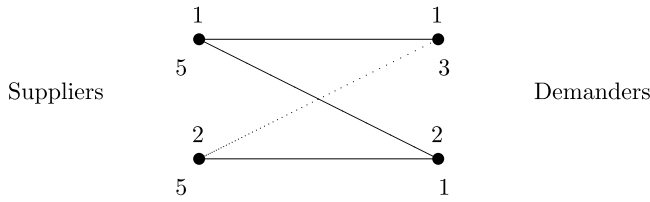
FIGURE 5. A new link may hurt noninvolved agents.
