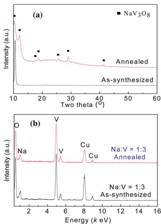
Fig. 1 (a) XRD patterns of the as-synthesized nanobelts and the annealed nanobelts at 400 °C in air and (b) EDS spectra of the as-synthesized nanobelts and the annealed nanobelts at 400 °C in air.
