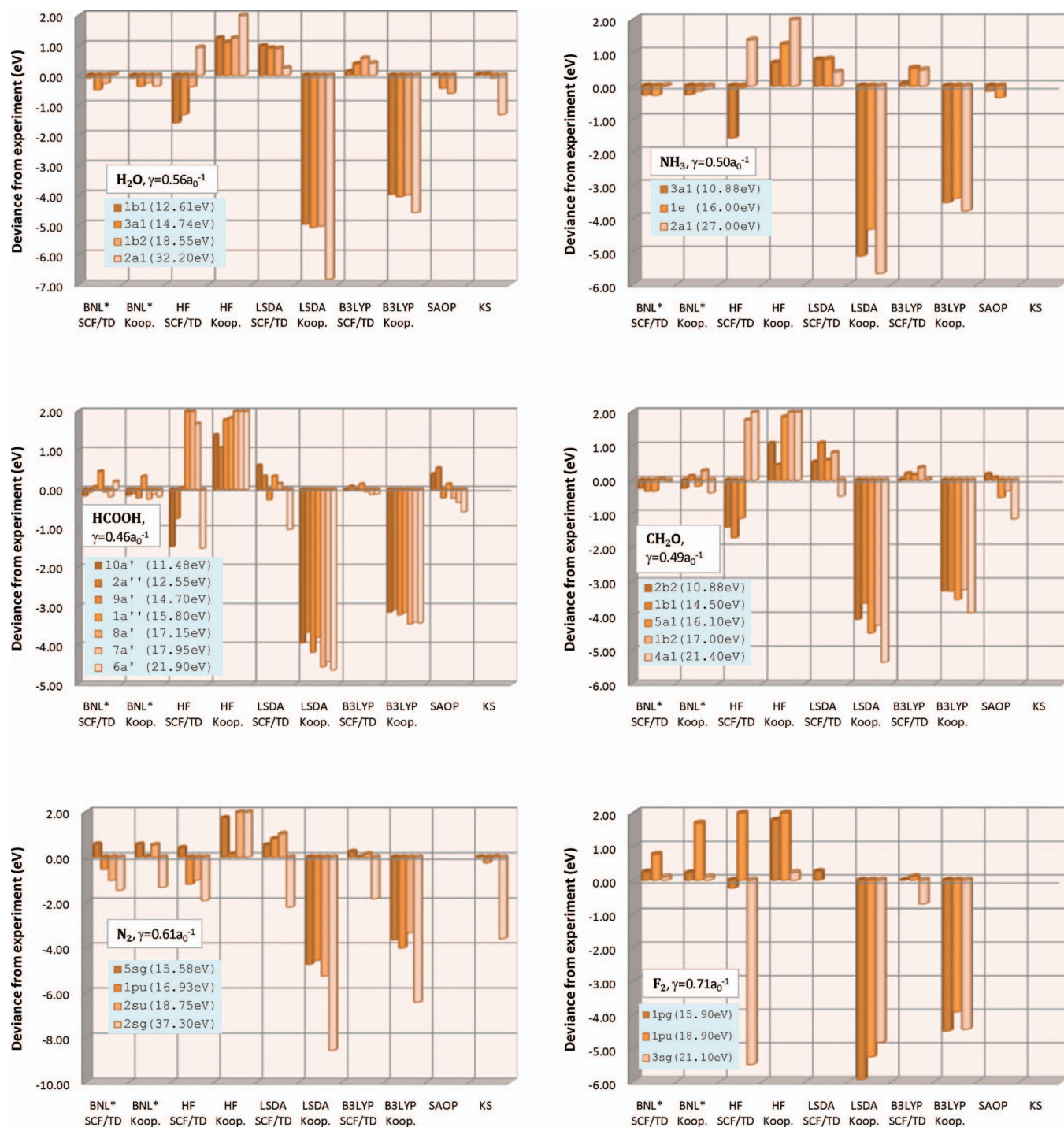
FIG. 1. Deviance of negative OOs and SCF/TD energies relative to vertical IPs derived from experimental data (Refs. 50–52) for several molecules. KS and SAOP OOs data are taken from Ref. 9.
