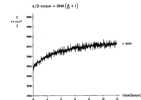
Fig. 5. Digitized output of the z axis of the ENTRAN accelerometer shown along with the fitted model of form C_1(1 - e^{-t/T}) + C_2 . Data was collected over a period of 12 hours by sampling every minute when the z axis was subject to gravity.
