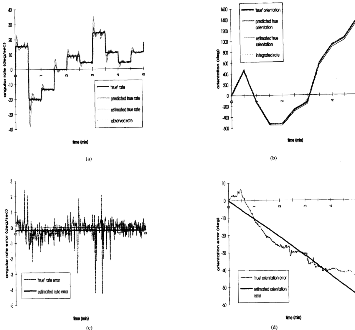
Fig. 10. (a) Angular rate and (b) position of the Gyrostar when nonzero input was applied. A new angular rate was randomly generated every 30 s and applied to the gyro. The true values and the erroneous observations are displayed along with the EKF results which compensate for the error. (c) Error in the angular rate and (d) error in orientation. Both the true and the estimated values are shown.
