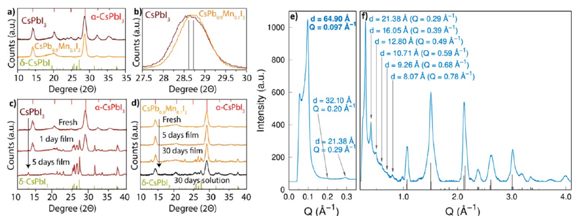
Figure 83. (a) XRD patterns of CsPbI 3 and Mn 2+ -substituted phase. The calculated \alpha - and \delta -phase patterns are shown in red and green, respectively. (b) Zoom in of (a) to visualize the shift in Bragg peak position due to Mn 2+ -induced lattice parameter changes. (c,d) Time-dependent XRD patterns of CsPbI 3 and CsPb 0.9 Mn 0.1 I 3 over several days, showing the difference in degradation kinetics. Reproduced from ref 607. Copyright 2017 American Chemical Society. (e,f) Low- and high-angle XRD pattern of CsPbBr 3 nanoplatelets. The first peak corresponds to a distance of the NPs of 6.5 nm. Higher harmonics are also visible, which confirms the high degree of long-range order. The NPs have a thickness of around 3.5 nm, as confirmed by TEM imaging. From the high-angle region, an orthorhombic structure could be determined. Reproduced from ref 210. Copyright 2019 American Chemical Society.
