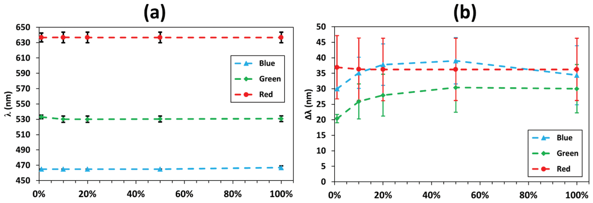
Fig. 4: Average and standard deviations of the (a) peak emission wavelengths ( \lambda ) and (b) full-width at half-maximum ( \Delta\lambda ) values of the spectra that acquire the lowest 1%, 10%, 20%, 50% and 100% values of f_{\text{circadian}} .
