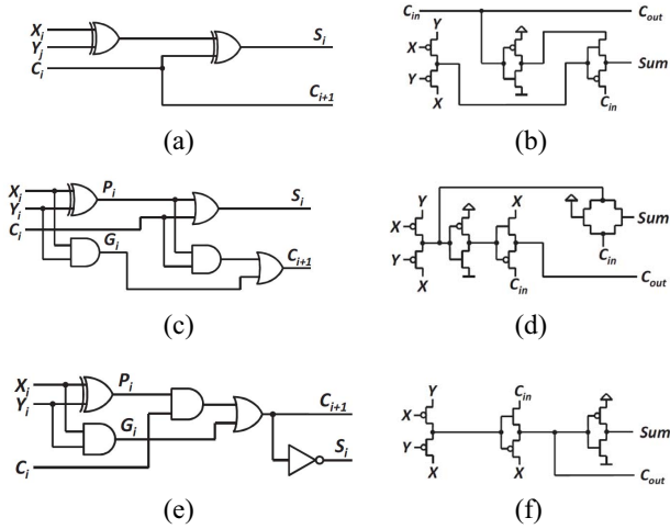
Fig. 1. Three considered inexact adder cells proposed in [1]. Logic diagrams of (a) InXA1, (c) InXA2, and (e) InXA3. Transistor circuit diagrams of (b) InXA1, (d) InXA2, and (f) InXA3.
