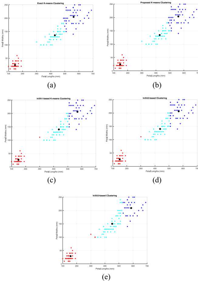
Fig. 7. K -means clustering results. (a) Exact K -means clustering. (b) K -means clustering with the proposed multiplier. (c) K -means clustering with the InXA1-based multiplier. (d) K -means clustering with the InXA2-based multiplier. (e) K -means clustering with the InXA3-based multiplier.
