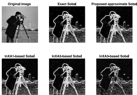
Fig. 8. Original image and the Sobel Filter implementations for: exact implementation, proposed multiplier, InXA1, InXA2, and InXA3.
