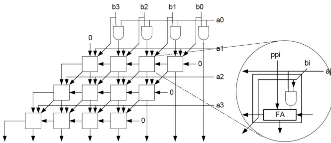
Fig. 2. 4 \times 4 multiplier architecture.
