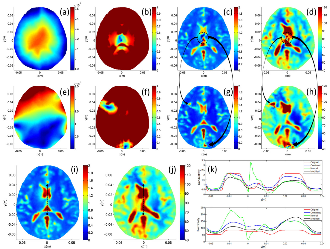
Figure 10. Head model results: ((a) and (e)) B_1^+ magnitude, ((b) and (f)) F_x magnitude, ((c) and (g)) conductivity reconstructions ( S\ m^{-1} ), ((d) and (h)) relative permittivity reconstructions for the normal and modified drive respectively, (i) combined conductivity reconstruction, (j) combined relative permittivity reconstruction and (k) profile plots of original conductivity and relative permittivities (red) as well as profile plots of the reconstruction results for the normal drive (green), modified drive (black) and combined reconstruction (blue) cases. The profiles are taken along the dashed lines in (i) and (j).
