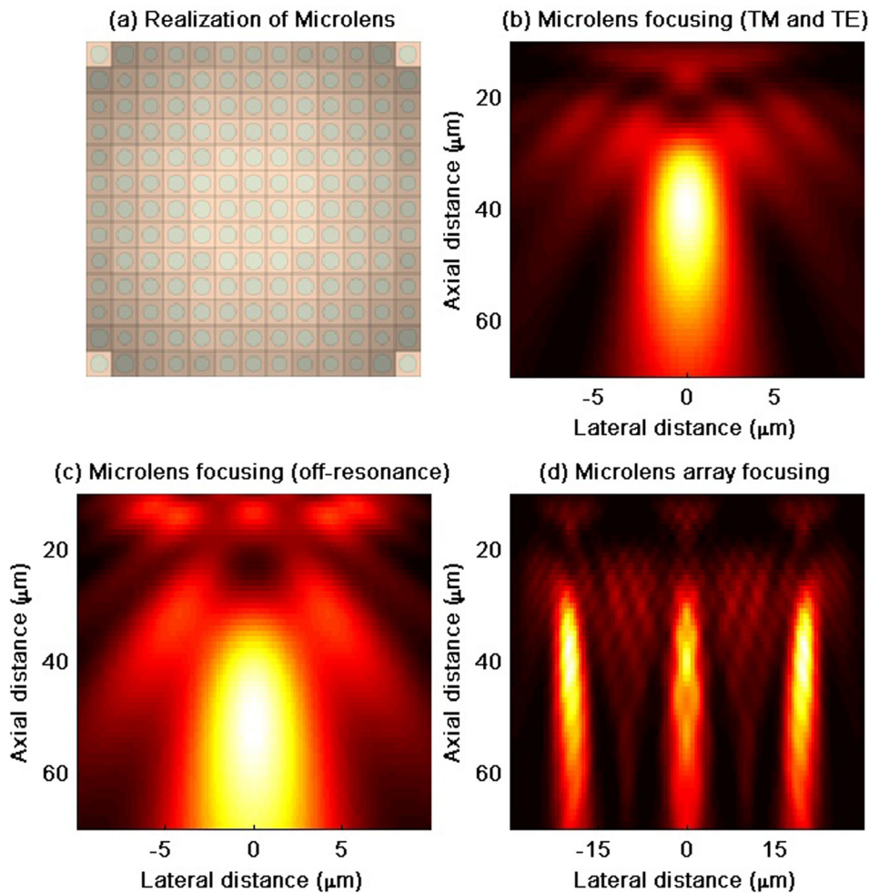
FIG. 2. (a) Realization of the optimized design's central microlens by Si nanodisks (the color of unit cells is graded within constant phase regions). (b) Far-field intensity distribution of light focused by the central microlens of the optimized design when excited with either TM or TE polarized light. (c) Far-field intensity distribution of light focused by the central microlens of the optimized design for the off-resonance wavelength of 3.5 \mu\text{m} which is different from the on-resonance design wavelength. (d) Far-field intensity distribution of light focused by different pixels of the optimized microlens array design.
