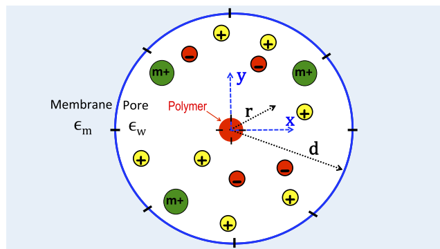
FIG. 1. Schematic representation of the polyelectrolyte with line charge density \tau located on the axis of the cylindrical nanopore. The pore has radius d and fixed negative surface charge density \sigma_m . The polymer portion inside the pore has length l_p . The membrane and pore dielectric permittivities are, respectively, \epsilon_m = 2 and \epsilon_w = 80 .
