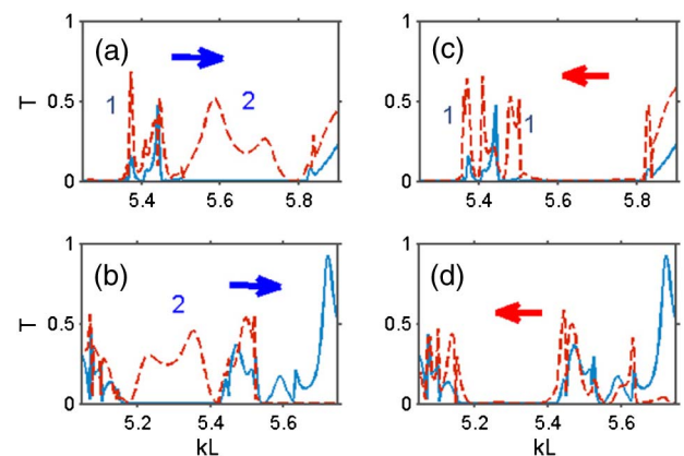
Fig. 11. Transmittance versus kL for structures with irregular layers ( p = L = 2a ) that is the fourth layer from the upper interface, which are illuminated from (a), (b) upper side and (c), (d) lower side. (a), (c) d/a = 0.5 , (b), (d) d/a = 0.55 , \varepsilon = 9.61 , and \theta = 47^\circ . Solid blue line, t_0 ; dashed red line, (a), (b) t_{-1}^{\rightarrow} and (c), (d) t_{-1}^{\leftarrow} .
