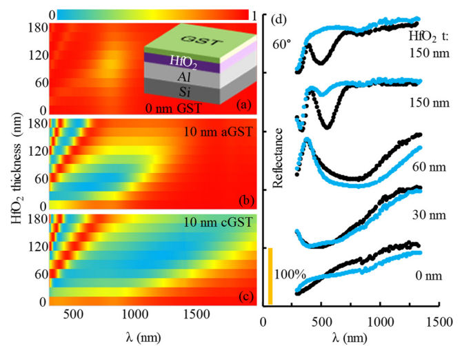
FIG. 4. The effect of the HfO 2 layer between GST and Al layers. Calculated reflection spectra for varying thickness of HfO 2 on Al (a) without GST and with (b) 10 nm aGST and (c) 10 nm cGST top layers. (Inset) Illustration of the structure. (d) Measured reflection spectra of 10 nm aGST (black) and 10 nm cGST (blue) top layers on HfO 2 films with indicated thicknesses. The curves are shifted along the y-axis. The angle of incidence for the top curves is 60° and 30° for the rest.
