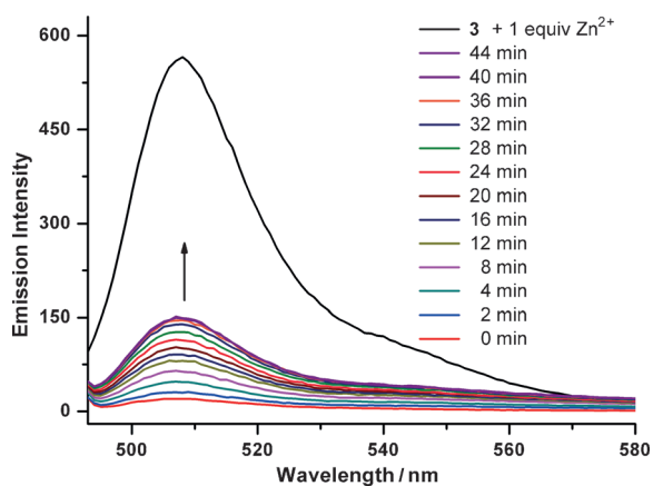
Figure 4. Emission spectra showing the fluorescence response of compound 3 (DPA-BOD) after uncaging of 1 + \text{Zn}^{2+} ( 5.0 \mu\text{M} each) by light irradiation (recorded in \text{CH}_3\text{CN} ). Time values indicate the duration of irradiation with the Xe lamp (wavelengths of higher energy than \lambda = 400 \text{ nm} filtered out). Irradiation results in the photolysis of the \text{Zn}^{2+} complex 1 + \text{Zn}^{2+} and is followed by an increase in emission intensity due to the formation of the 3 + \text{Zn}^{2+} complex ( \lambda_{\text{ex}} = 490 \text{ nm} ). Highest intensity emission trace represents the maximum emission intensity of 3 (DPA-BOD) obtained by the addition of 1.0 equivalents of zinc(II) ions in the form of the triflate salt.
