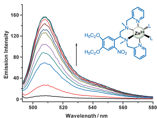
Figure 6. Emission spectra showing the fluorescence response of compound 3 after uncaging of one equivalent of o -nitrobenzyl \text{Zn}^{2+} cage complex ( 5.0 \mu\text{M} each) by light irradiation (recorded in \text{CH}_3\text{CN} ). Compound 3 (DPA-BOD) initially exhibits no fluorescence (quenched due to the active PET process). As the solution was irradiated at \lambda = 360 \text{ nm} (for 10 min) the increase in the emission intensity levels off, which can be interpreted as the completion of photolysis of the \text{Zn}^{2+} cage compound.
