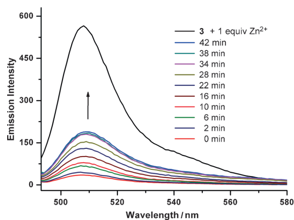
Figure 5. Emission spectra showing the fluorescence response of compound 3 (DPA-BOD) after uncaging of 2 + \text{Zn}^{2+} ( 5.0 \mu\text{M} each) by light irradiation (recorded in \text{CH}_3\text{CN} ). Time values indicate the duration of irradiation with the Xe lamp (wavelengths of higher energy than \lambda = 400 \text{ nm} filtered out). Compound 3 initially exhibits low fluorescence (quenched due to the active PET process). Irradiation results in the photolysis of the 2 + \text{Zn}^{2+} complex and is followed by the enhanced emission intensity of 3 ( \lambda_{\text{ex}} = 490 \text{ nm} ). Highest intensity emission intensity represents the maximum emission intensity of 3 (DPA-BOD) obtained by the addition of 1.0 equivalents of zinc(II) ions in the form of the triflate salt.
