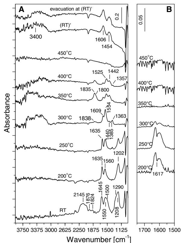
Figure 4. Panel A: FT-IR spectrum of the sample Pd/WZ containing adsorbed \text{NO}_x species (spectrum (RT), see the caption of figure 1 for the conditions) and spectra taken upon heating in \text{CH}_4 (60 Torr) for 20 min at the indicated temperatures and after cooling to room temperature (RT) followed by evacuation. Panel B: Spectra of the gas phase detected at the indicated temperatures (RT = room temperature).
