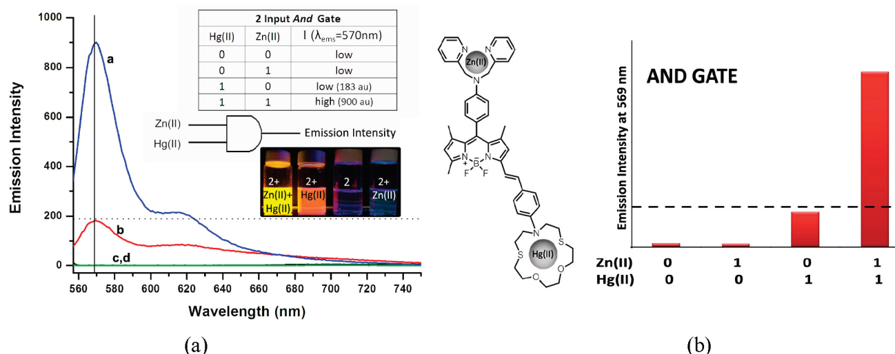
Figure 2. Emission spectra of 2 (1.67 \mu\text{M} ) in acetonitrile in the presence of Hg(II) and Zn(II) (6.68 and 1.67 \mu\text{M} , respectively). Inset shows truth table for AND gate ( \lambda_{\text{ex}} = 555 \text{ nm} ).
