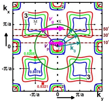
FIG. 1. (Color online) IFCs at a/\lambda=0.5078 (nearly square blue contours), a/\lambda=0.5205 (nearly square green contours) and a/\lambda=0.5321 (nearly square red contours). The boxed numbers on the IFCs, 2 and 3, correspond to the second and third lowest bands of the PC. Thin arrows show possible directions of group velocity, \mathbf{v}_g . The PC interface is along \Gamma -X direction (dotted black line). Air band (circle-shaped green contour around \Gamma point), the incident wave vectors ( \mathbf{k}_0 , intermediately thick dark turquoise arrows), the phase velocities ( \mathbf{v}_p , intermediately thick purple arrows), the directions of \mathbf{v}_g (thick pink arrows), and the construction lines (dashed wine-colored straight lines) at \psi=10^\circ , 30^\circ , and 50^\circ are shown for a/\lambda=0.5078 . The IFCs are marked with solid geometrical shapes (blue triangle for a/\lambda=0.5078 , green circle for a/\lambda=0.5205 , and red square for a/\lambda=0.5321 ).
