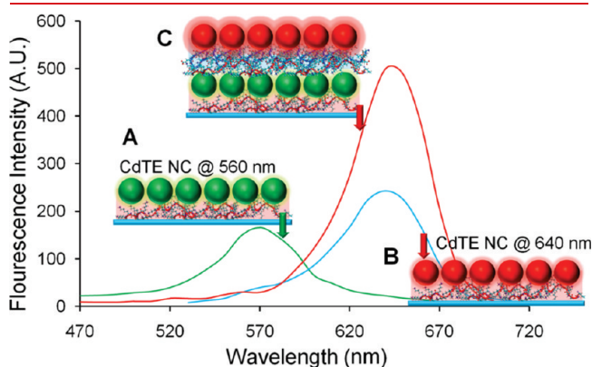
Figure 5. Steady-state photoluminescence (PL) of individual CdTe QDs emitting at 560 nm (the donor alone) assembled in the peptide film (A), steady-state PL of individual CdTe QDs emitting at 640 nm (the acceptor alone) assembled in the peptide film (B), and steady-state PL collectively from both CdTe QDs emitting at 560 nm and those emitting at 640 nm (the donor–acceptor pair) in the same peptide film, showing the strong modification in the PL intensity of these QDs through FRET (C).
