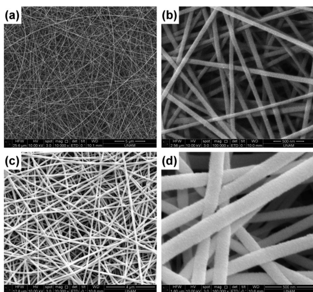
Fig. 1 Representative SEM images of (a) and (b) pristine nylon 6,6, and (c) and (d) nylon–GaN core–shell nanofibers at different magnifications.
