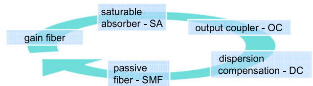
Fig. 1 Illustration of the fiber laser cavity elements used for the simulations
