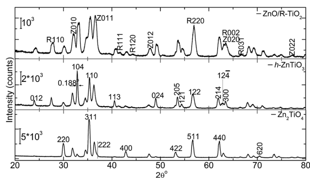
Fig. 4 XRD patterns of nanotube titanates ZT14, ZT13 and ZT12. For ZnO/ R-TiO}_2 additional planes (104), (110), (113) and (121) from h-ZnTiO}_3 phase were not annotated.
