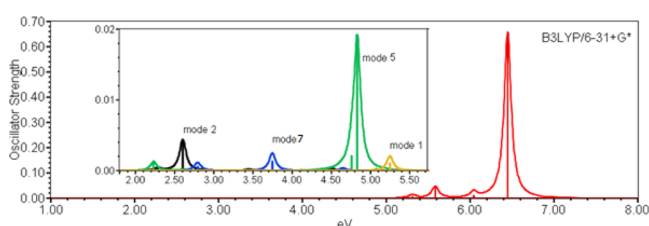
Figure 5. UV spectrum of ferrocene in vibrational ground and excited states at the B3LYP/6-31+G* level of theory.
