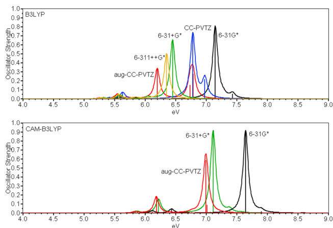
Figure 2. Effect of basis set enlargement on the UV spectrum of eclipsed (D5h) ferrocene with the B3LYP and CAM-B3LYP functionals.
