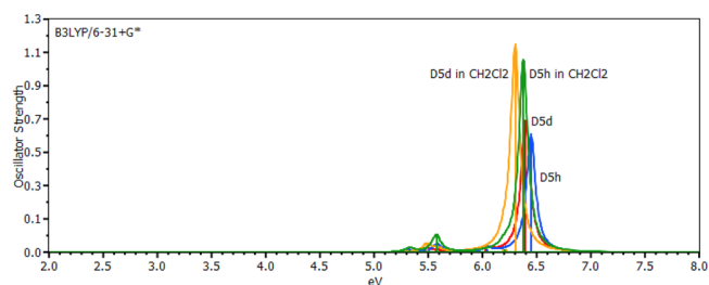
Figure 1. UV spectra of gas phase and methylene dichloride solution spectra of eclipsed (D5h) and staggered (D5d) ferrocene at the B3LYP/6-31+G* level of theory.
