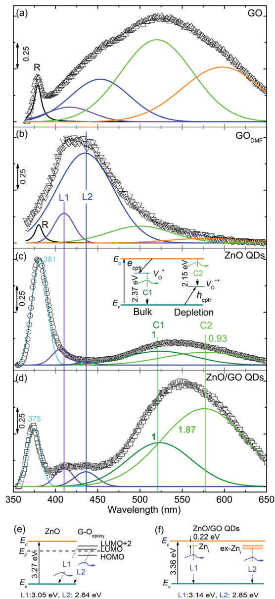
Fig. 6 Fluorescence from (a) GO, (b) \text{GO}_{\text{DMF}} , PL/optical emission from (c) ZnO QDs, (d) ZnO/GO QDs, (e) schematic of the two emission lines redrawn after Son et al. 3 and (f) ZnO/GO QDs with defect levels \text{Zn}_i and \text{ex-Zn}_i states, insert of (c) depicts the schematic of the green emission from ZnO. Area ratio is indicated with reference to that of 524 nm the (C1) peak in the respective sample. E_c , E_v are conduction and valance bands, respectively, while e_{\text{cptr}} and h_{\text{cptr}} are electron and hole capture processes, respectively, and E_F is the Fermi level. L1 and L2 on part (b) only indicate the spectral overlap of the emission peaks and hence should not be attributed to \text{Zn}_i s and \text{ex-Zn}_i s.
