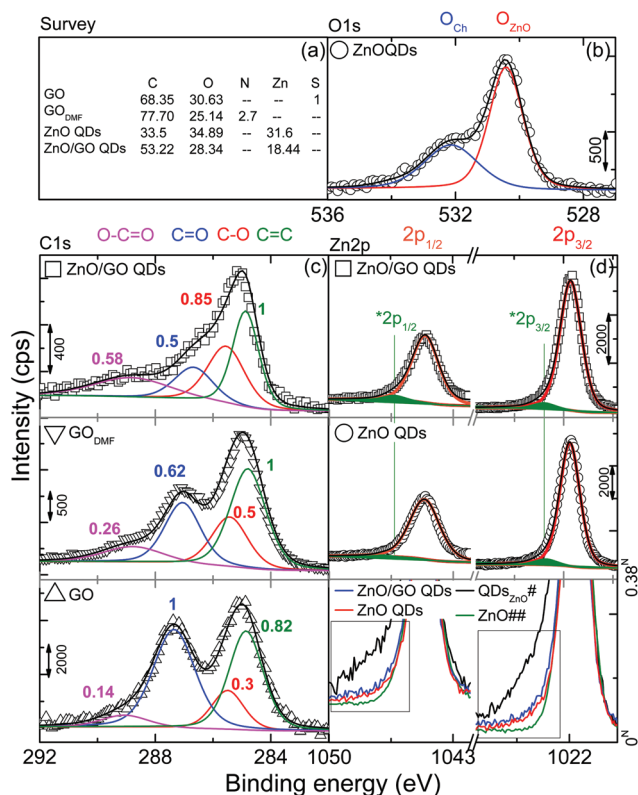
Fig. 4 (a) Atomic %, (b) O 1s from ZnO QDs, (c) C 1s from GO, GO_{DMF} , ZnO/GO QDs and (d) Zn 2p from ZnO QDs, ZnO/GO QDs, normalized plot compares with ZnO. Data taken from the # ref. 17 and ## ref. 32. N normalized intensity scale.
