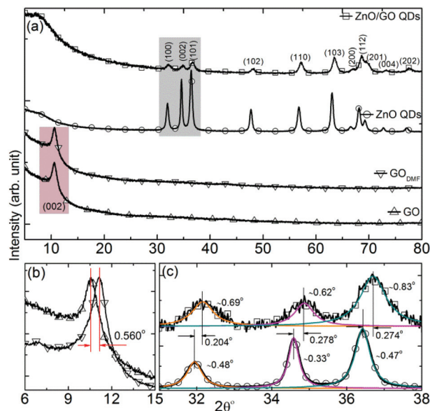
Fig. 3 XRD patterns from (a) GO, \text{GO}_{\text{DMF}} , ZnO QDs, ZnO/GO QDs (b) GO, \text{GO}_{\text{DMF}} ( 6-15^\circ ) and (c) ZnO QDs, ZnO/GO QDs ( 31-38^\circ ) with the fwhm values and angular shifts annotated.
