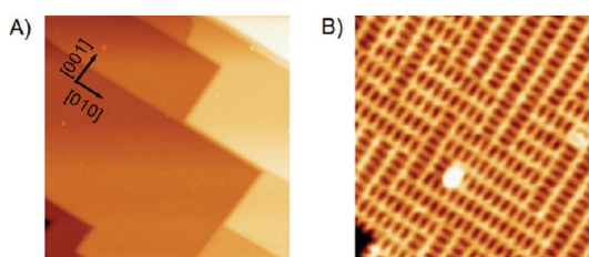
Figure 2. Experimental STM images of the Cu(100)–O surface. (A) Large-scale image (75 nm \times 75 nm) revealing the step-edge pinning along the [010] and the [001] directions. (B) High-resolution image (9 nm \times 9 nm) illustrating orthogonal domains also oriented along the [010] and [001] directions; note that domains may be as small as two unit cells. Imaging parameters: (A) +1.0 V/0.9 nA; (B) –1.1 V/0.4 nA.
