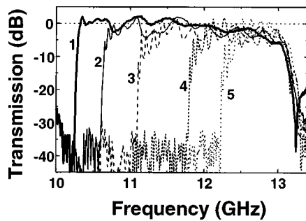
FIG. 2. Transmission amplitude measured from parallel-plate waveguides as the separation width of the waveguide is changed. The numbers given in the plot are assigned to width of the guides as (1) 18, (2) 16, (3) 14, (4) 12, (5) 10.5 mm.
